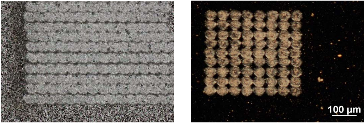
Fig. 2. Marking results without facer fine delay offset adjustment (left) and after iterative calibration (right).
